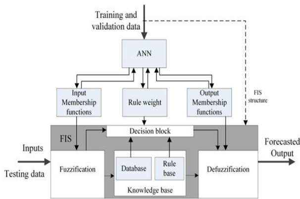
Fig. 1 fuzzy-neural inference system structure
