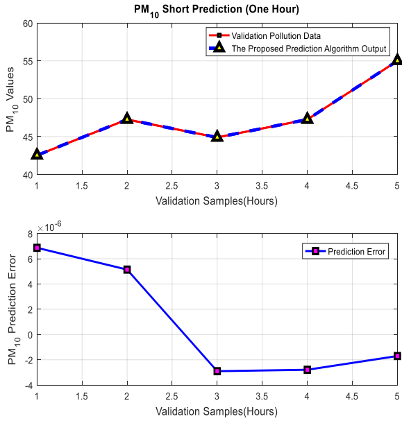
Fig. 8 system output and error for short-term prediction of validation data
