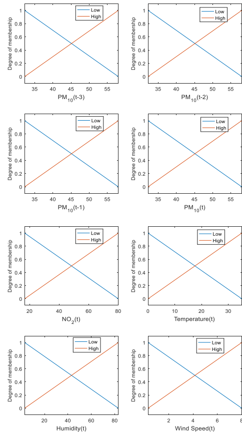
Fig. 4 membership functions related to 8 inputs
