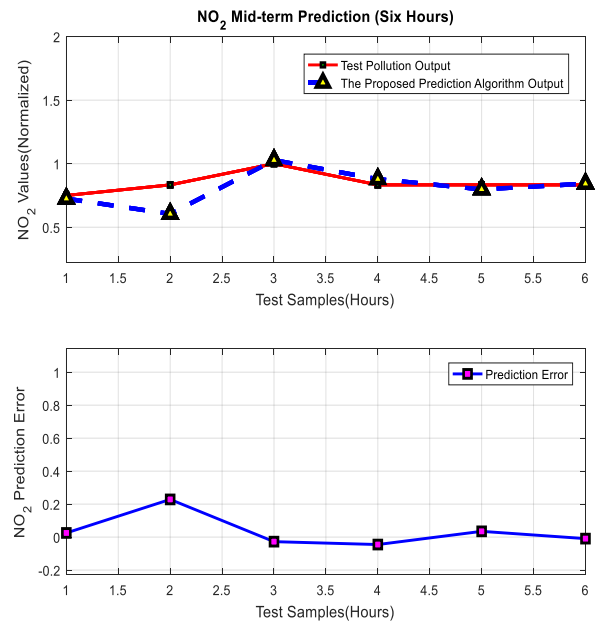
Fig. 11 system output and error for mid-term prediction of validation data
